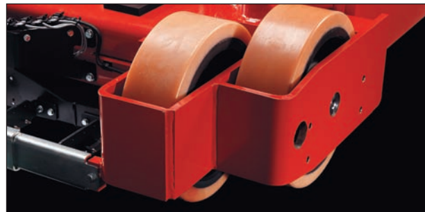
The VCE150A's staggered front wheels increase stability and reduce floor loading
